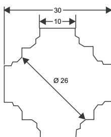
Bus Bar Dimension (mm) : 30 x 10, 20 x 25, Ø 26
